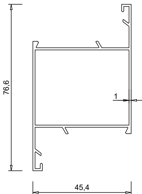
ALUM 1003 0.644 kg/m
