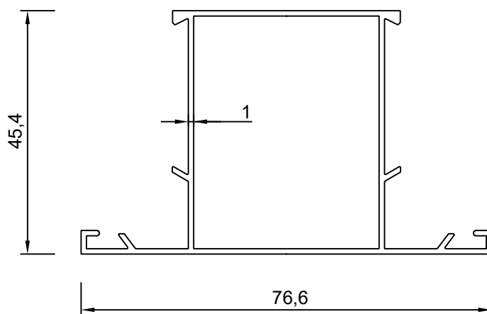
ALUM 1002 0.644 kg/m
