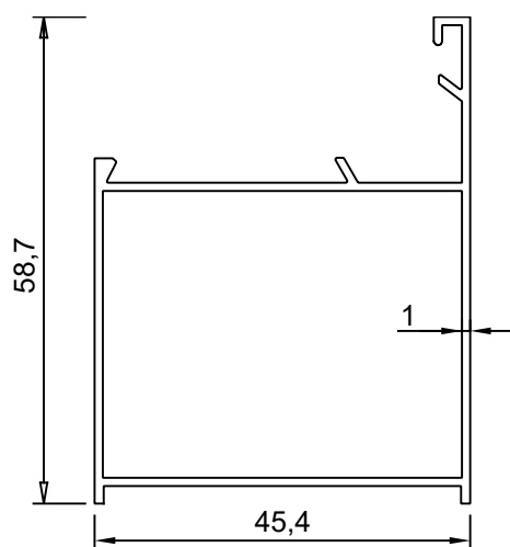
ALUM 1001 0.551 kg/m
