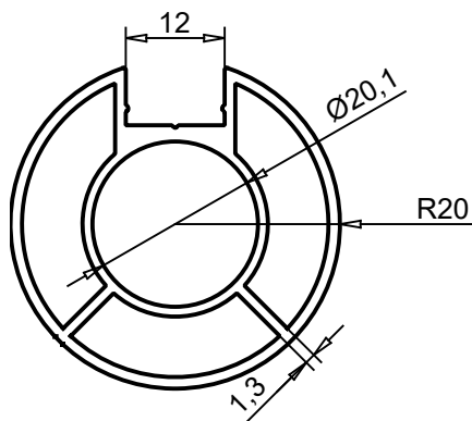
ALUM 2014 0.786 kg/m
