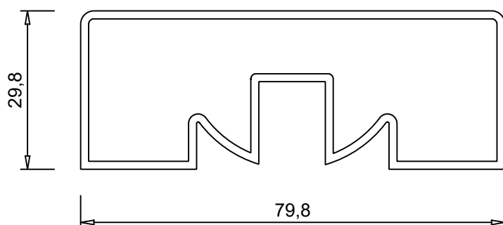
ALUM 2003 1.079 kg/m
