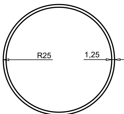
ALUM 2018 0.518 kg/m
