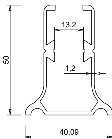
ALUM 2008 0.722 kg/m
