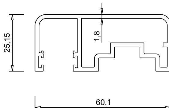
ALUM 2004 0.692 kg/m
