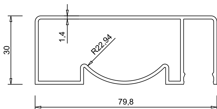
ALUM 2003 1.079 kg/m
