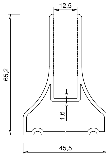
ALUM 2009 1.178 kg/m
