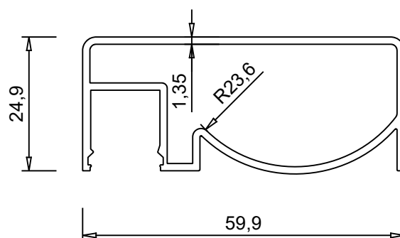
ALUM 2004 0.692 kg/m
