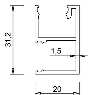
ALUM 2013 0.376 kg/m
