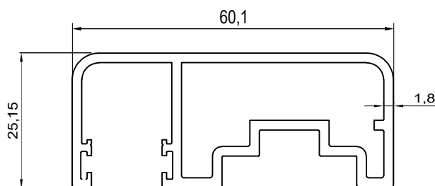
ALUM 2019 0.950 kg/m
