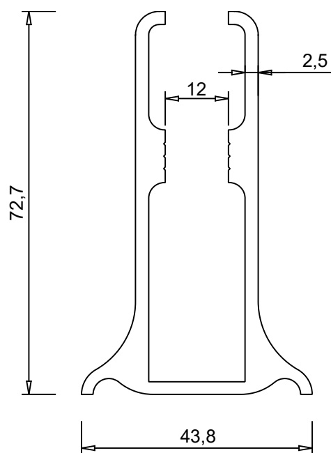
ALUM 2007 1.620 kg/m
