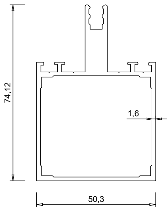
ALUM 5001 1.267 kg/m
