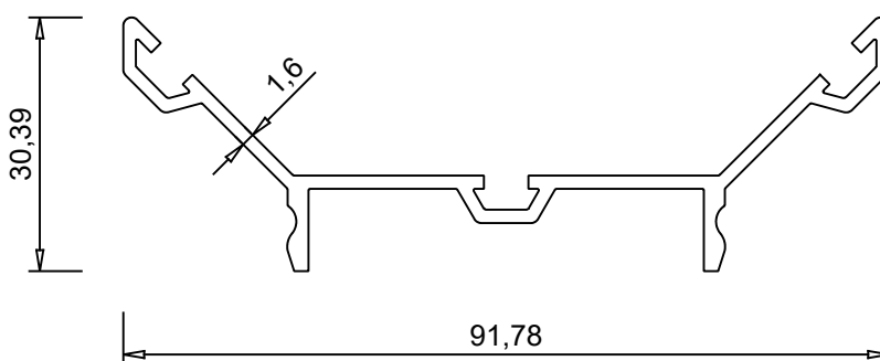
ALUM 5007 0.690 kg/m
