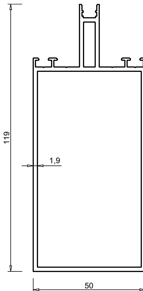
ALUM 5006 1.759 kg/m
