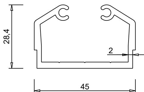
ALUM 5005 0.820 kg/m
