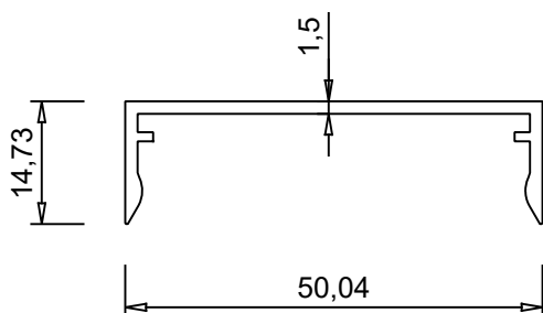
ALUM 5001 1.267 kg/m
