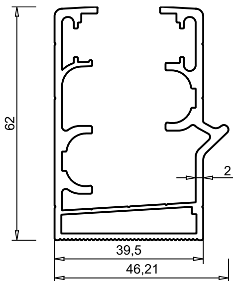
ALUM 10-001 1.393 kg/m
