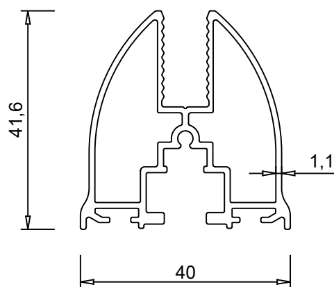
ALUM 10-003 0.726 kg/m
