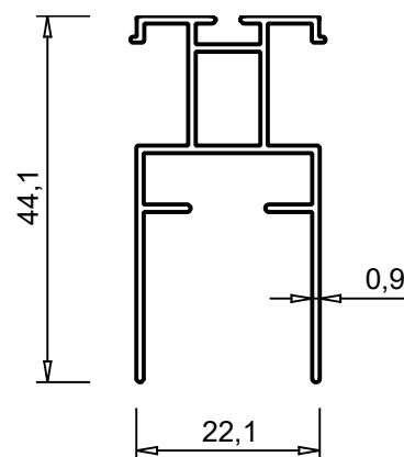
ALUM 10-009 0.366 kg/m
