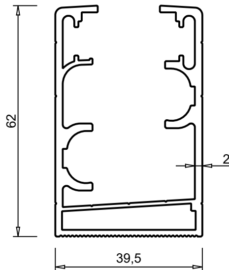
ALUM 10-002 1.350 kg/m
