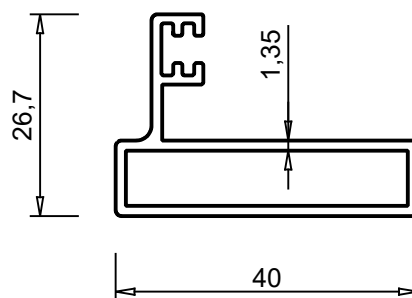
ALUM 10-004 0.466 kg/m
