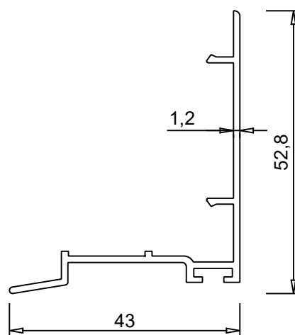
ALUM 3004 0.373 kg/m
