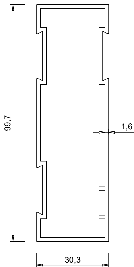
ALUM 3001 1.212 kg/m
