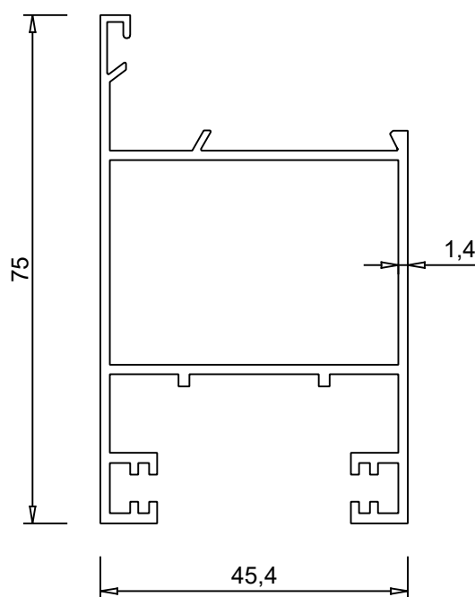
ALUM 3002 1.030 kg/m
