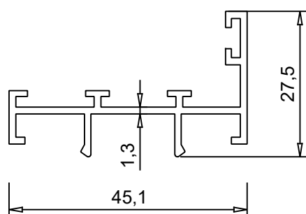
ALUM 3003 0.420 kg/m
